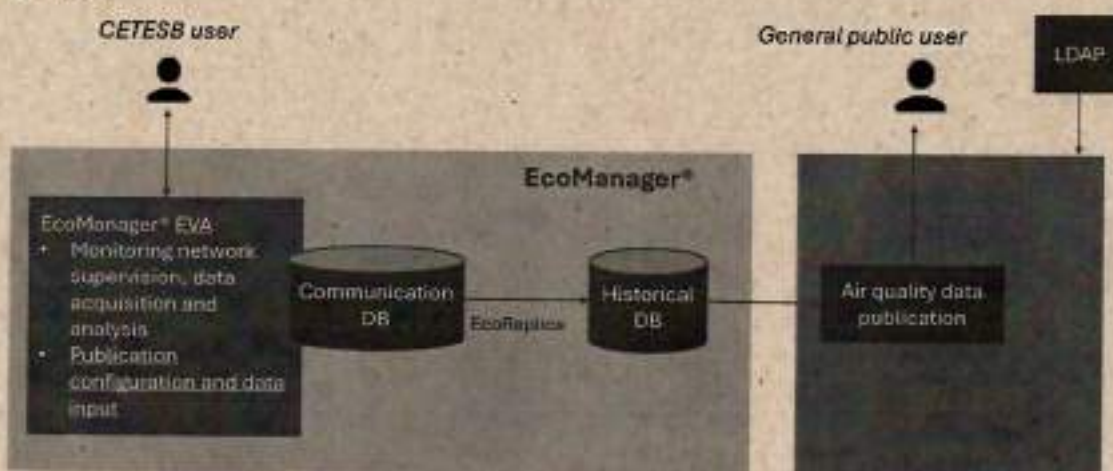
Figure 6 – Architecture of CETESB's air quality publication system – to be
