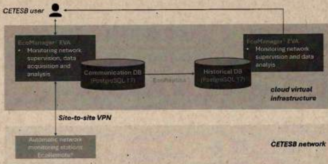
Figure 2 - Architecture - to be - Phase 1
