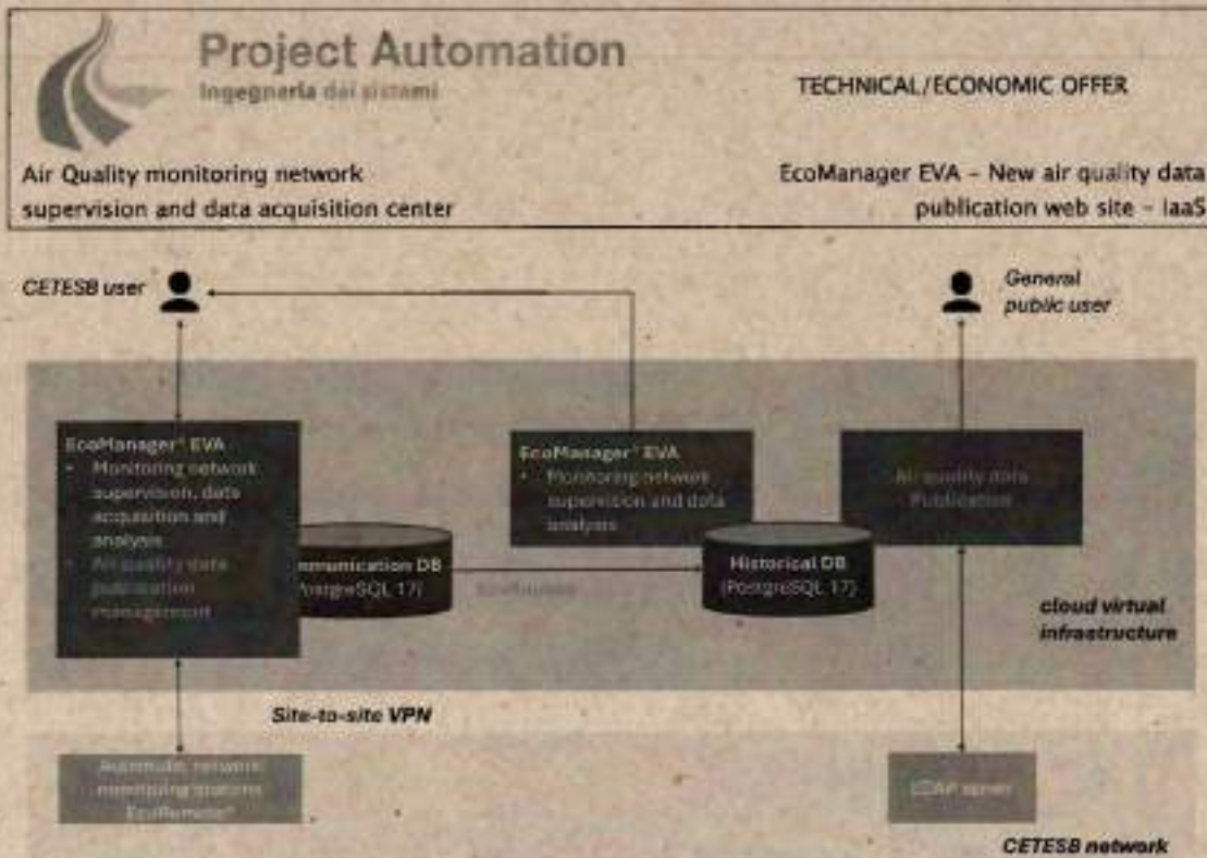
Figure 4 - Architecture - to be - Phase 2
