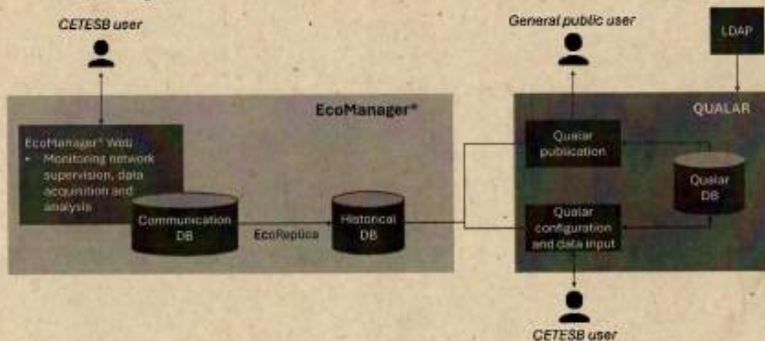
Figure 5 - Architecture of CETESB's air quality publication system - as is
